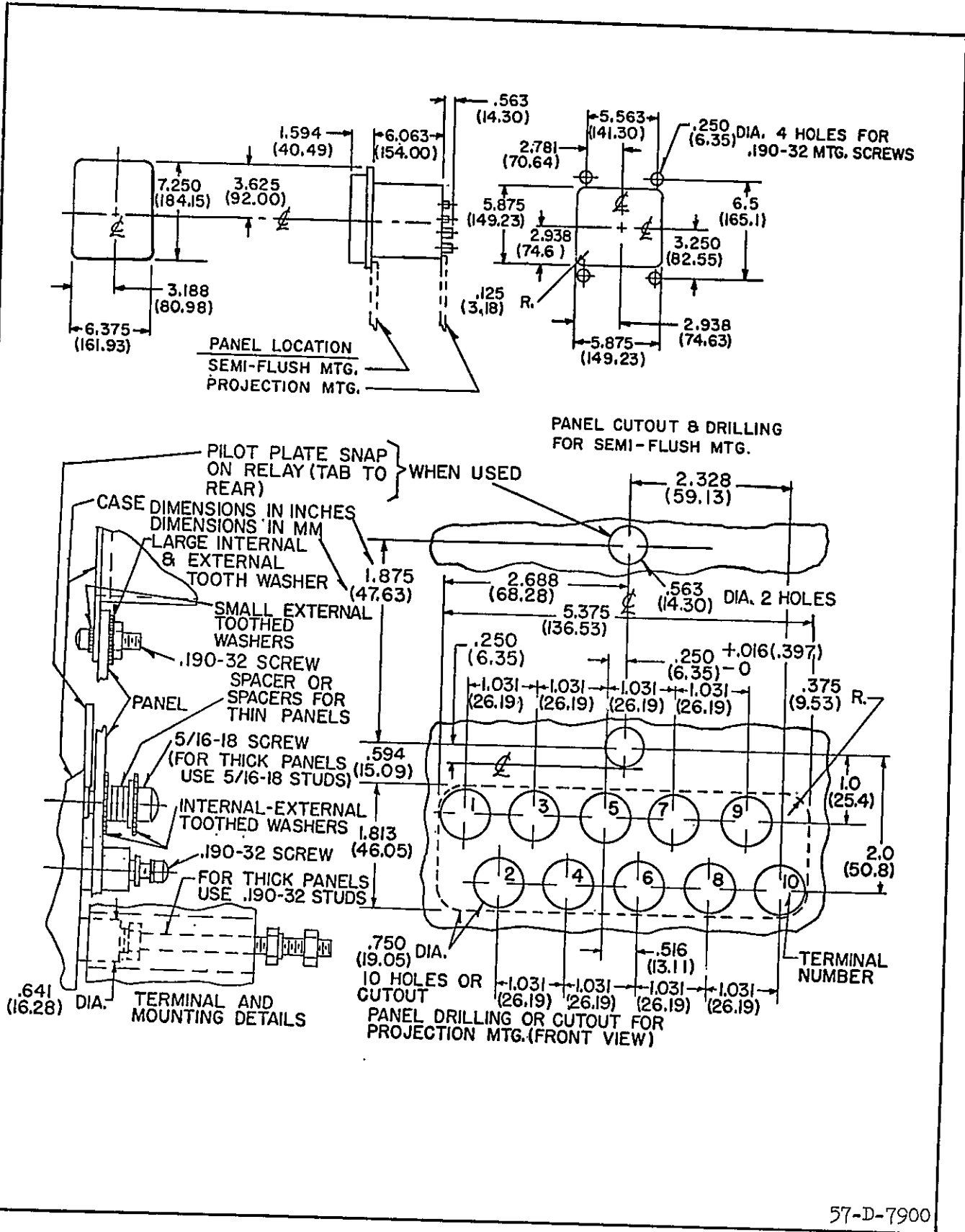
Fig. 7. Outline and Drilling Plan for the Type ITH Relay in the Type FT11 Case.
