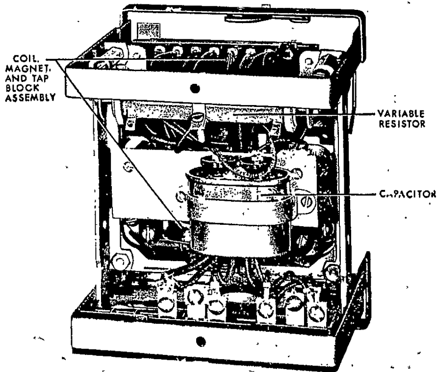
Fig. 1A (8035063) The Type IAC77B Relay Removed From Case (Rear View)
