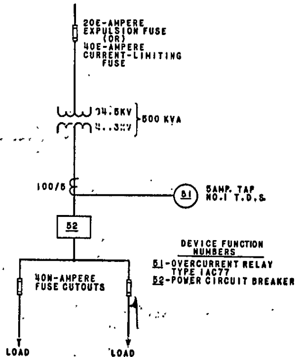
Fig. 3 (6507952-0) One-line Diagram Of Typical Distribution System Protected By Type IAC77 Time-Overcurrent Relay
