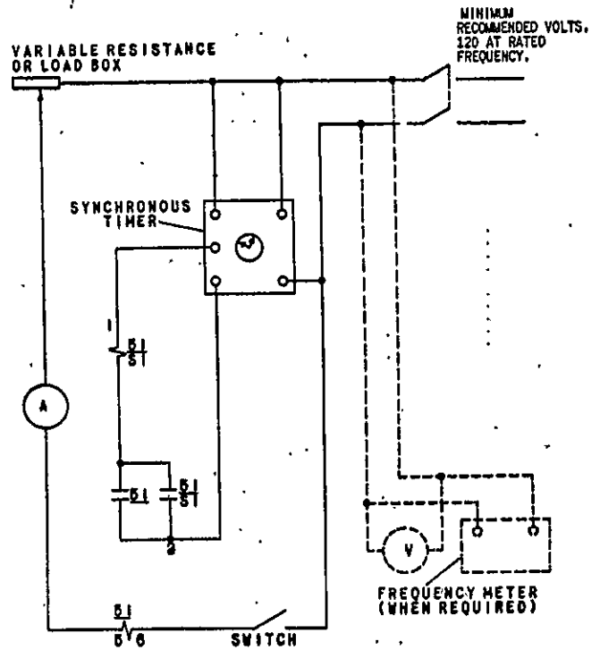
Fig. 8 (6154399-5) Connections For Testing Single-phase IAC Relay (Front View)
