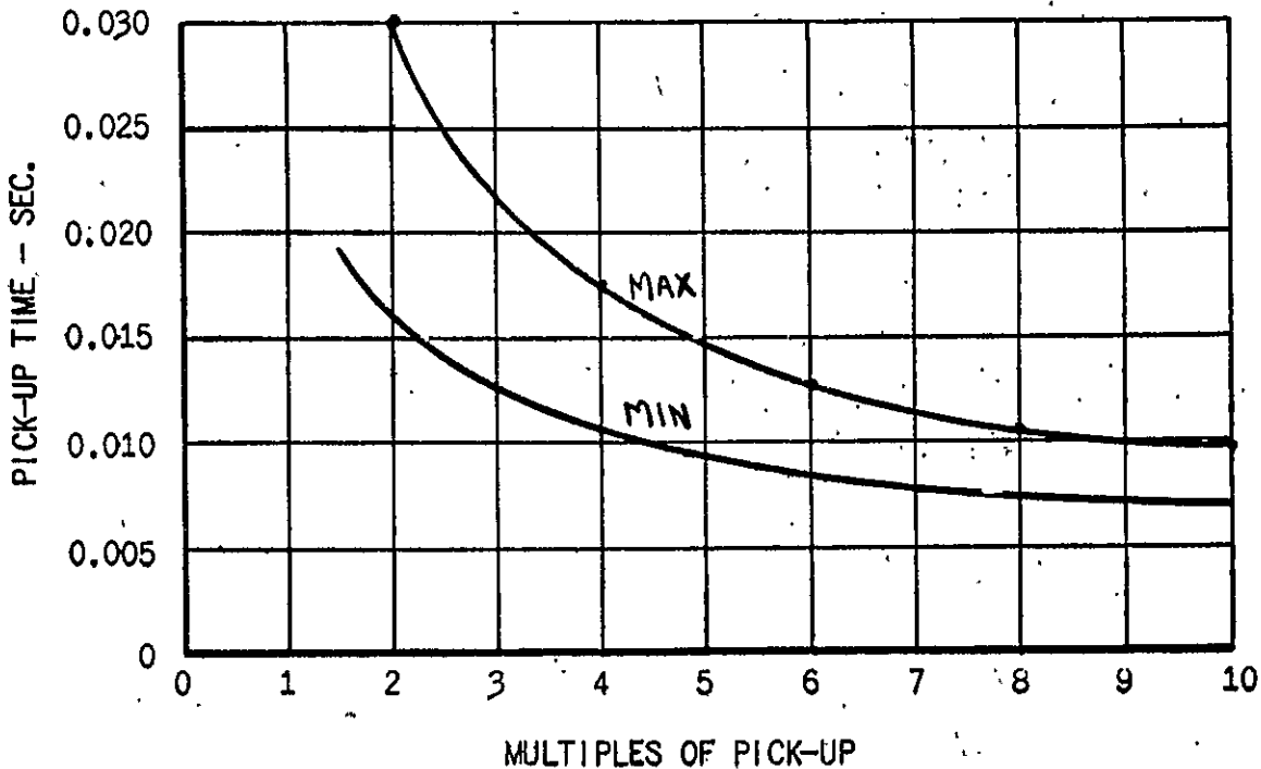
Fig. 9 (6306872-3) Time-Current Curve Of Instantaneous Unit
