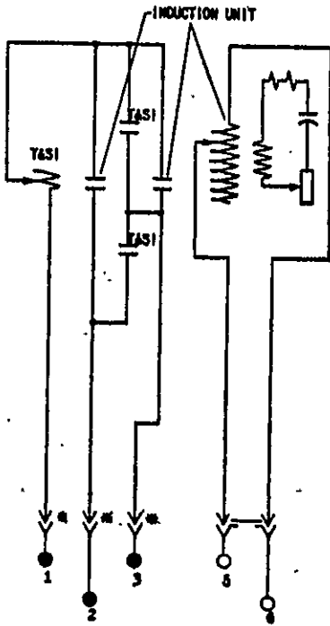
Fig. 10 (0165A7758-0) Type IAC77A Relay Internal Connections (Front View)
