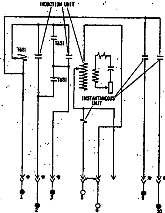
Fig. 11 (0165A7759-0) Type IAC77B Relay Internal Connections (Front View)
