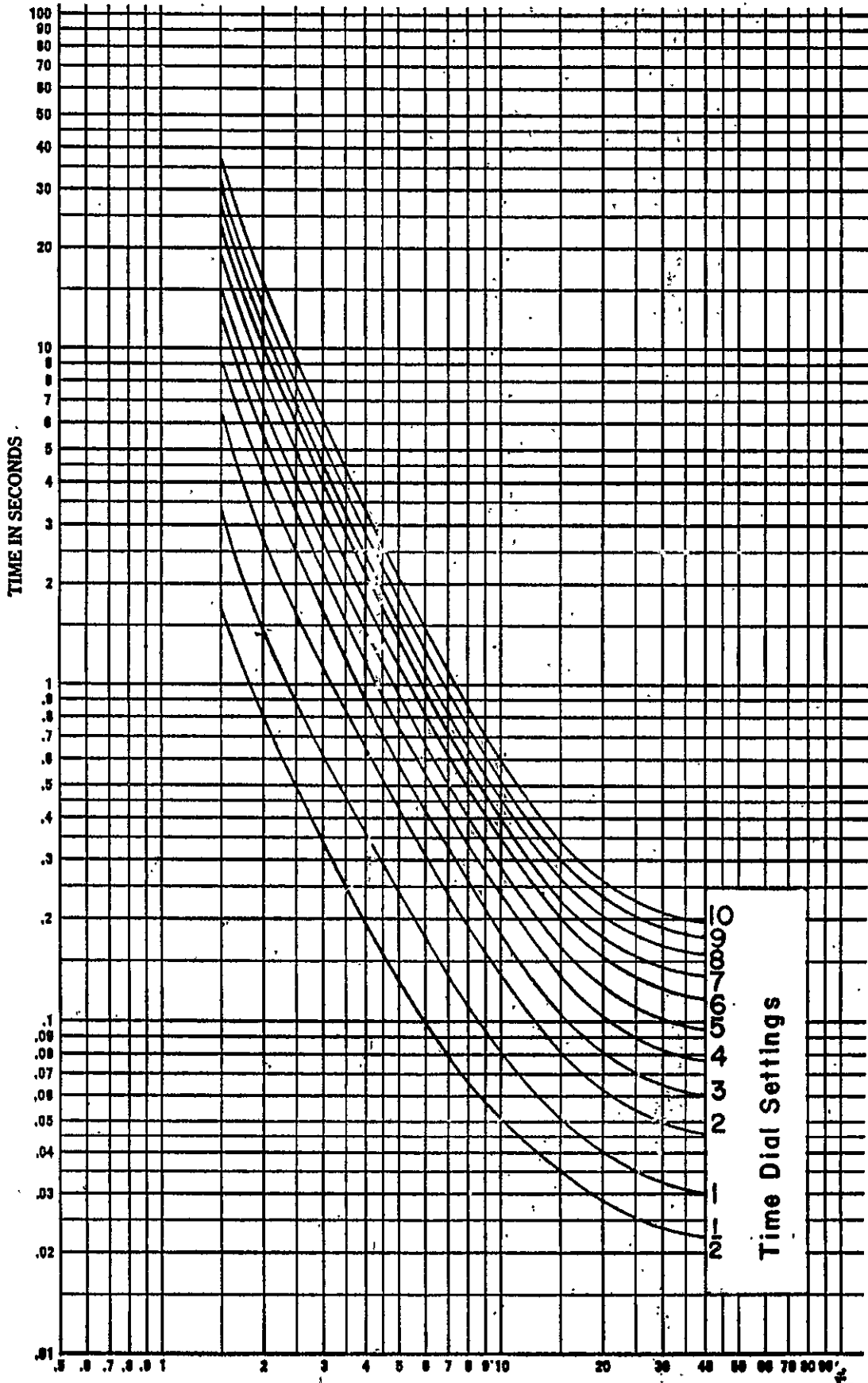
Fig. 6 (0888B0274-1) Time-current Characteristic For Type IAC77 And IAC78
