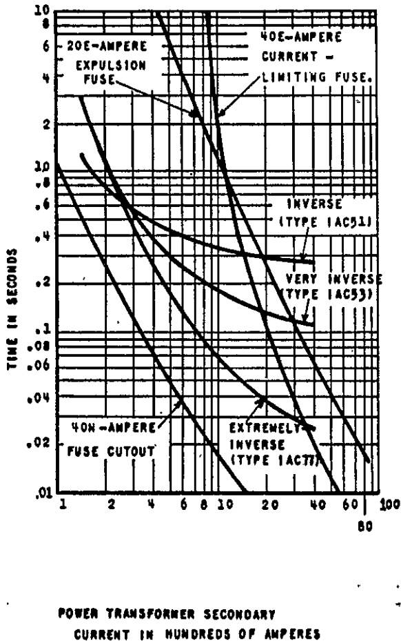
Fig. 2 (6507953-2) Comparison Of IAC Overcurrent Relay Characteristics Showing Co-ordination With Typical Primary And Secondary Fuses
