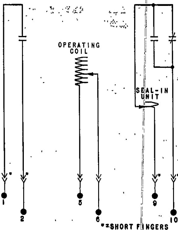
Fig. 1 Internal Connections For The Type IAV53F Relay (Front View)
