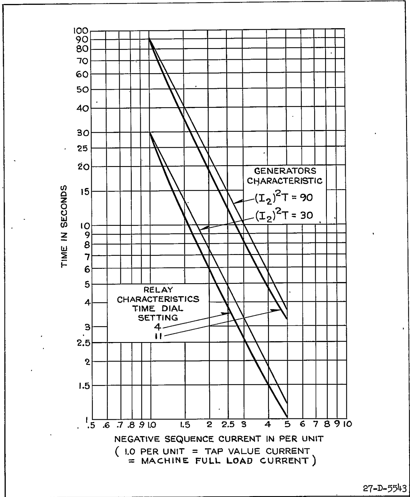
Fig. 5. Comparison of Relay and Generator Characteristics - Time Versus Negative-Sequence Current, For an I_2^2 T Factor From 30 to 90.
