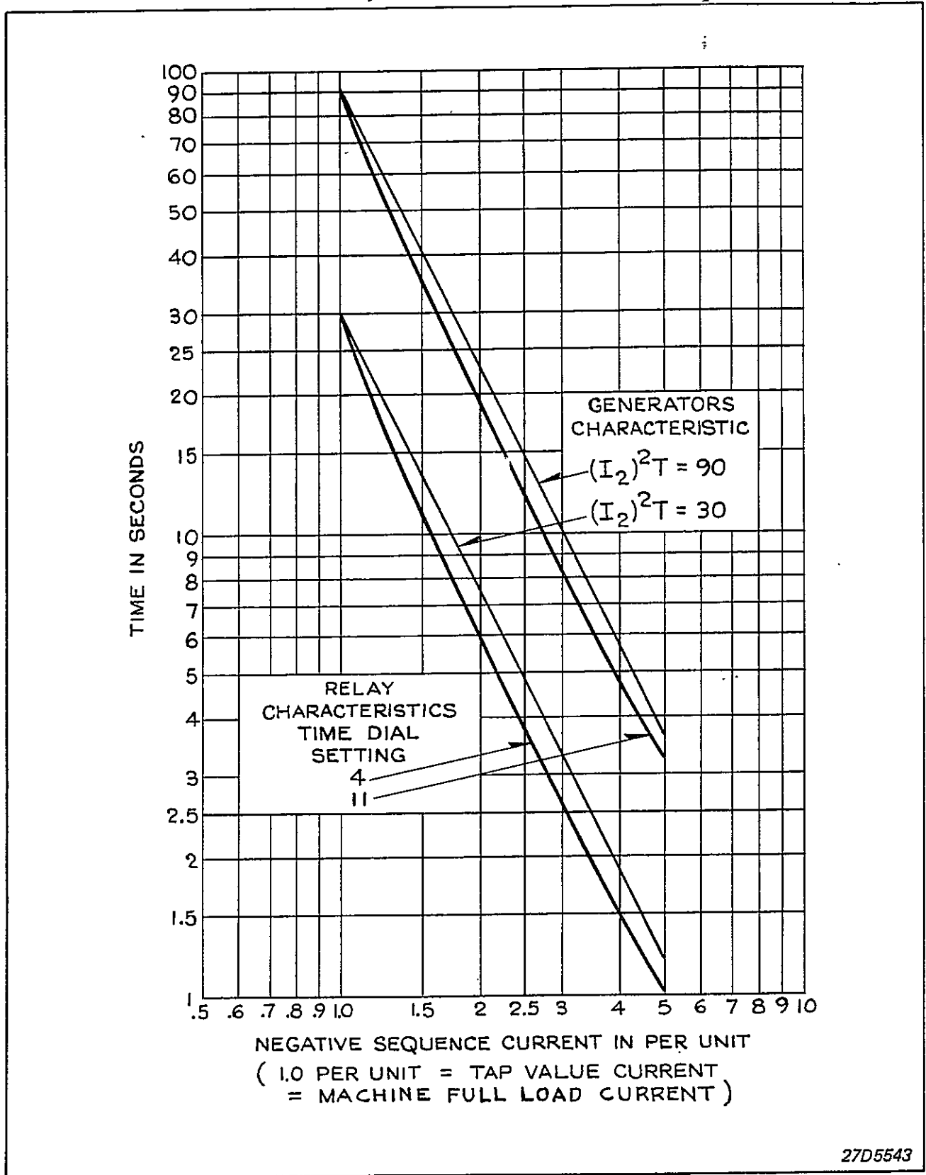
Fig. 5. Comparison of Relay and Generator Characteristics — Time versus Negative Sequence Current, for an I_2^2 T Factor from 30 to 90
