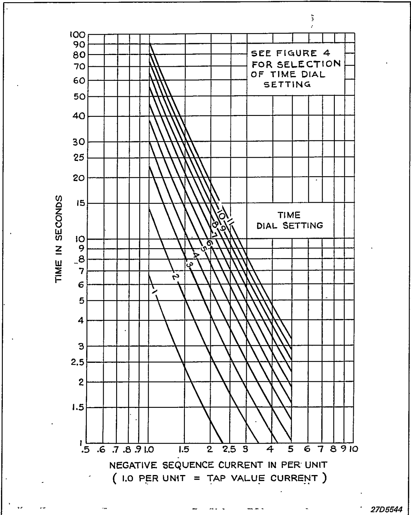
Fig. 7. Relay Time-Current Curve
