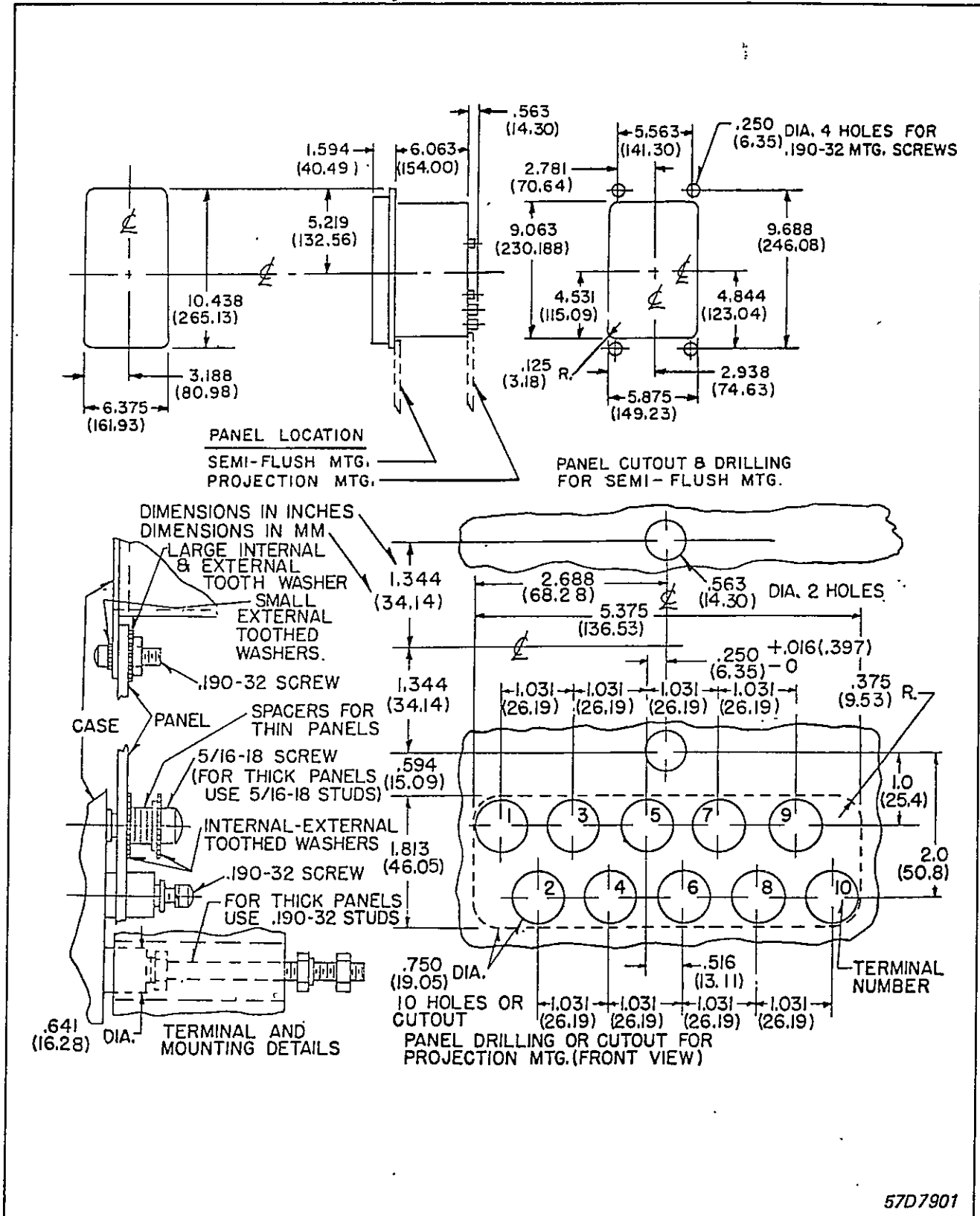
Fig. 11. Outline and Drilling Plan for the COQ Relay in the FT21 Case
