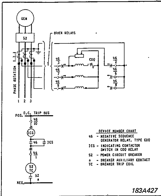
Fig. 8. External Schematic of the COQ Relay - Neutral Formed Within Relay
