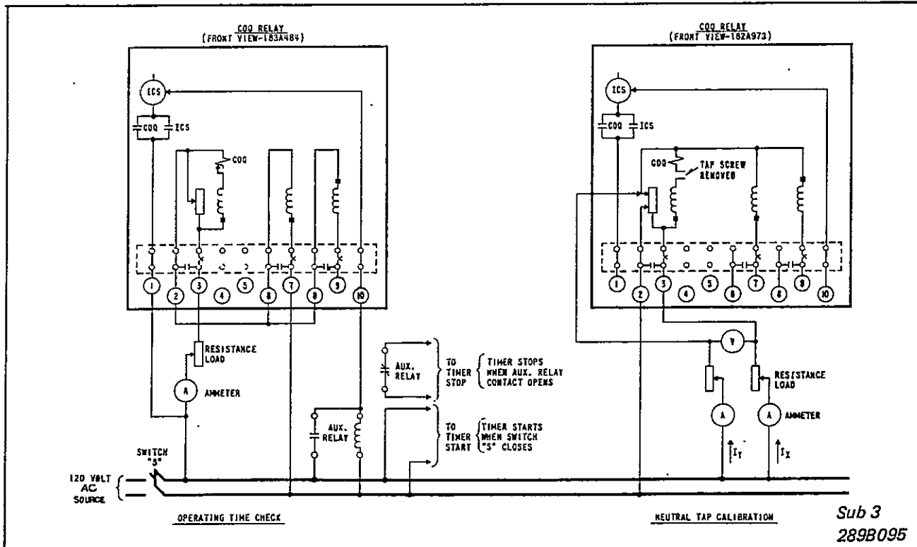
Fig. 10. Diagram of Test Connections for COQ Relay
