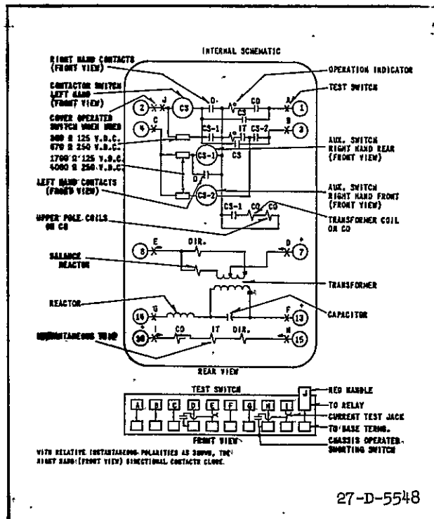
Fig. 4—Internal Schematic of the Single Trip Inverse, Very Inverse, or Short Time Type HCRD Relay With Instantaneous Trip to Separate Terminal in the Type FT Case.
