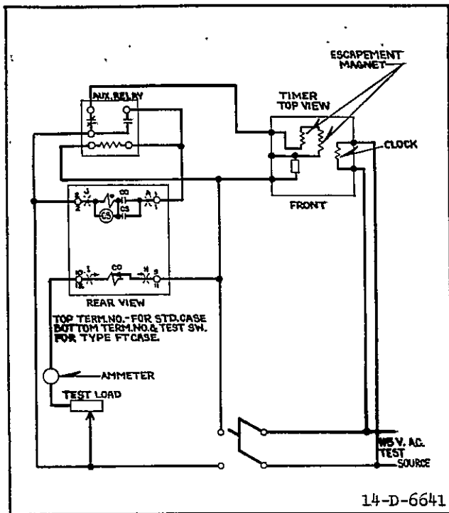
Fig. 8—Diagram of Test Connections of the Overcurrent Element.
