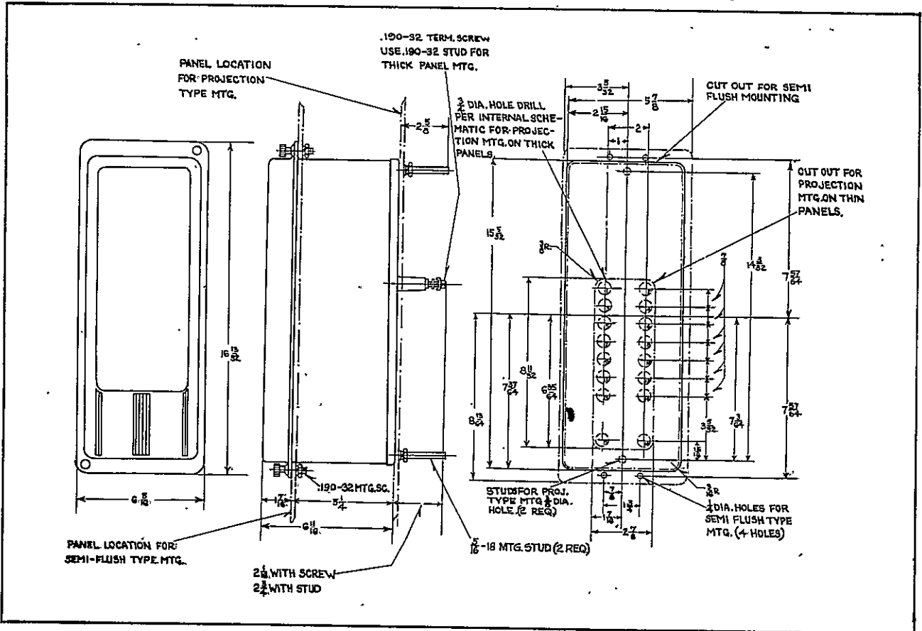
Fig. 11—Outline and Drilling Plan for MIO Projection or Semi-Flush Type FT Case.
