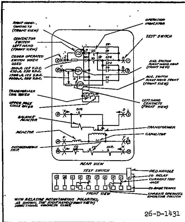
Fig. 2—Internal Schematic of the Double Trip Inverse, Very Inverse, or Short Time Type HCRD Relay With Instantaneous Trip in the Type FT Case.
