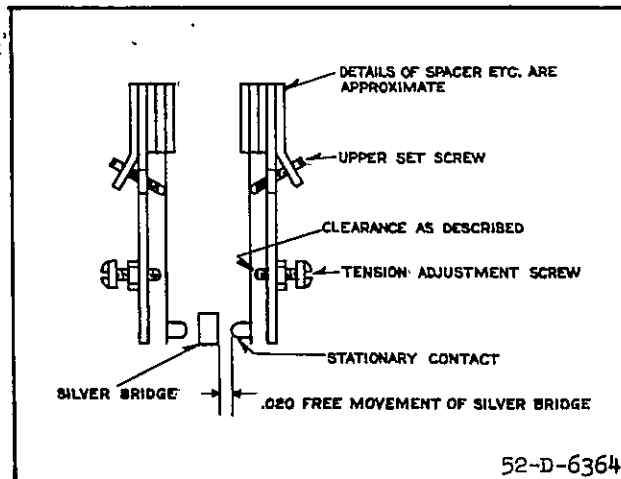
*Fig. 9—Front View of the Directional Element Showing Contact Adjustment Details.
