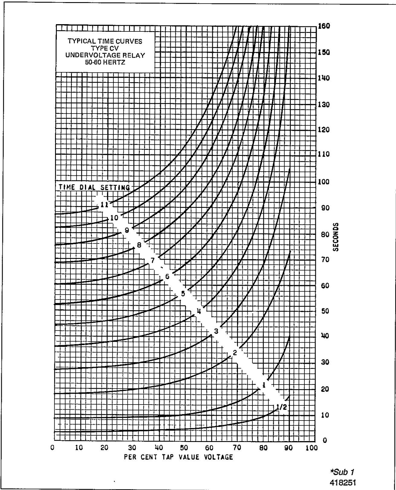
Figure 4. Typical Time Curves of the Type CV-21 Long Time Undervoltage Relay
