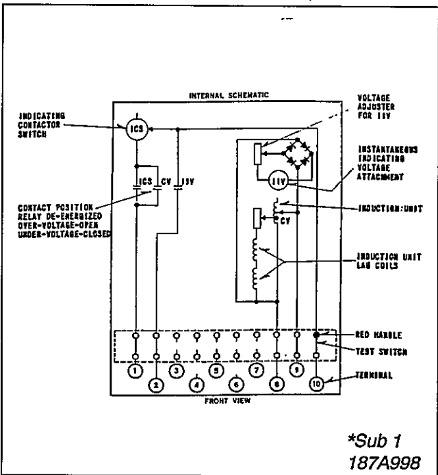
Figure 12. Internal Schematic for Type CV (S.P.S.T.) with Instantaneous Indicating Voltage Attachment in Type FT-11 Case
