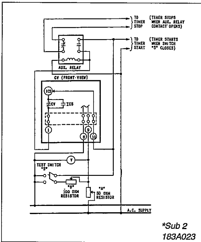
Figure 10. Diagram of Test Connections for Type CV Undervoltage Relays
