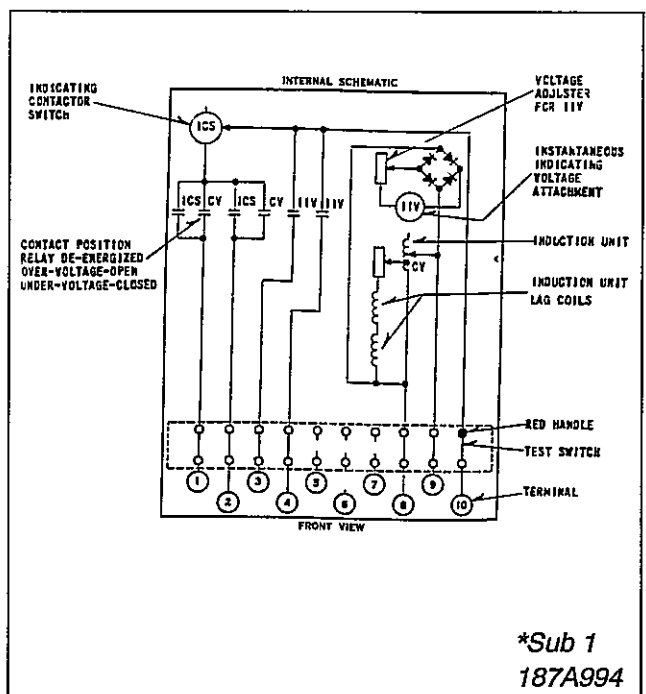
Figure 13. Internal Schematic for Type CV (D.P.S.T.) with Instantaneous Indicating Voltage Attachment in Type FT-11 Case
