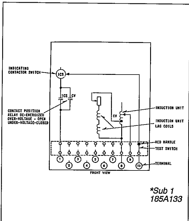
Figure 1. Internal Schematic for the Type CV (S.P.S.T.) Voltage Relay in the FT-II Case
