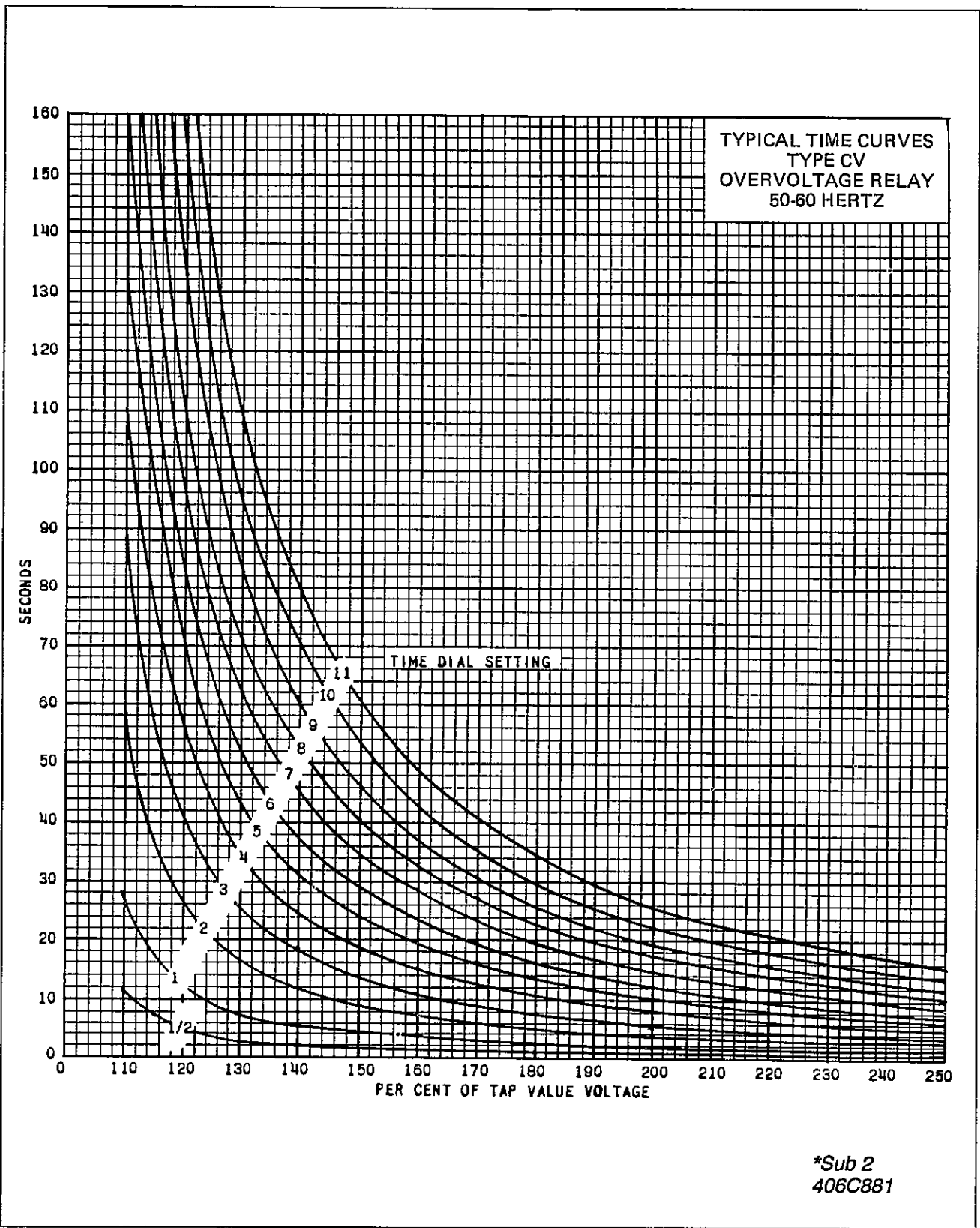
Figure 6. Typical Time Curves of the Type CV-24 Long Time Overvoltage Relay
