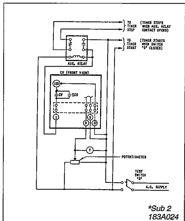
Figure 11. Diagram of Test Connections for Type CV Overvoltage Relays
