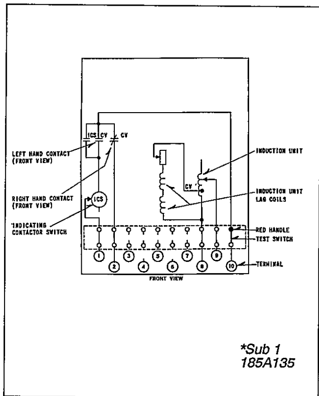
Figure 3. Internal Schematic for the Type CV (S.P.D.T.) Voltage Relay in the FT-11 Case
