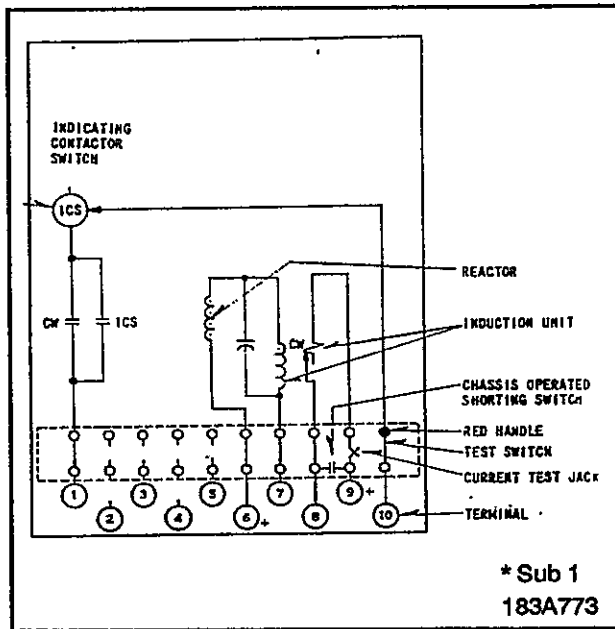
Figure 2. Internal Schematic of the Type CW Relay in the Type FT 21 Case.
