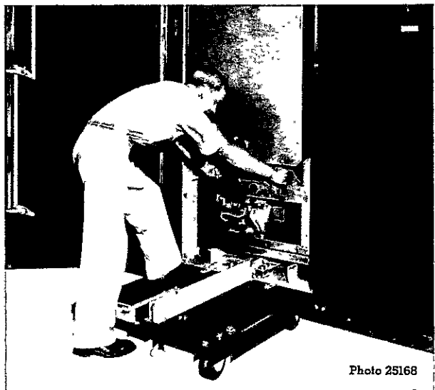
Fig. 4. To remove the circuit breaker, it must be first racked out into the test position, and unlocked. (See Instruction Bulletin on breaker). Then the breaker is pulled out as shown.
