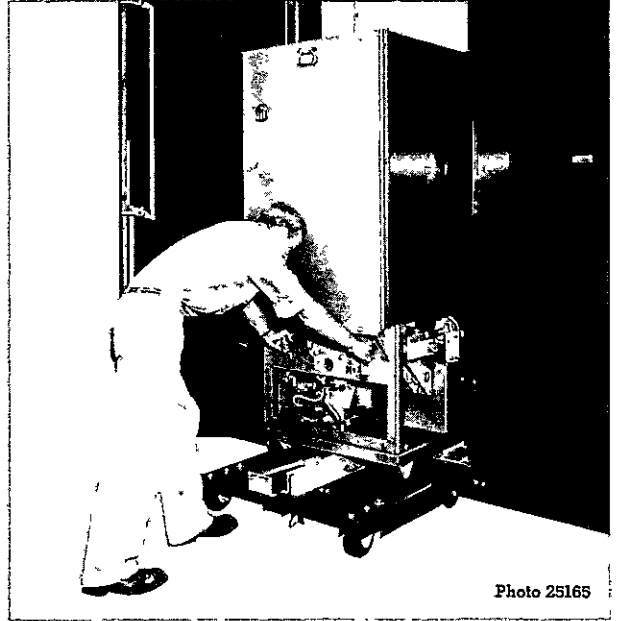
Fig. 7. To insert circuit breaker, move dolly against gear as described under Figs. 2 and 3. Then move breaker locking bar to the left and push breaker in as shown above.
