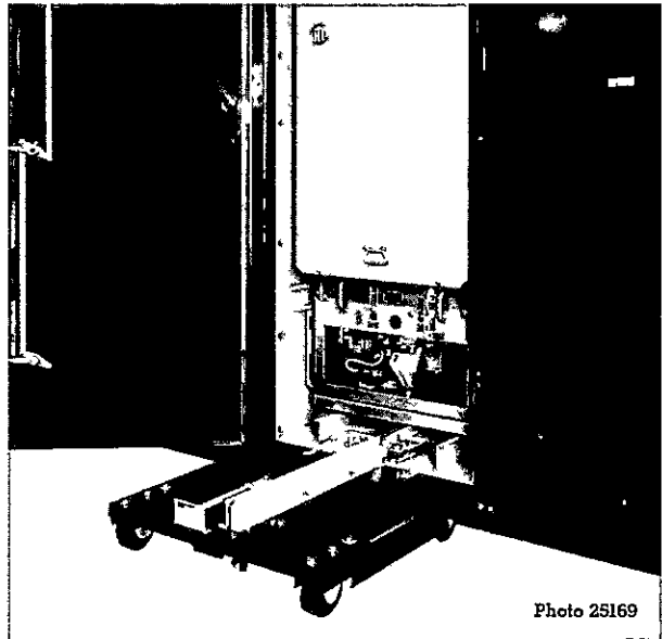
Fig. 3. After the dolly is aligned vertically and horizontally, it is pushed against the gear. Before attempting to move breaker out, make sure that the dolly locking bar is engaged, and pull dolly locking bar upwards, if necessary. Move breaker locking bar to the right.
