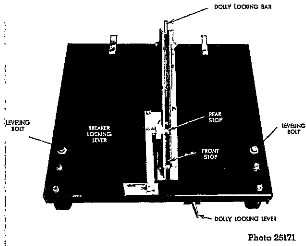
Fig. 1. A dolly like the one shown is furnished with each outdoor type 15HV metal-clad switchgear installation; to facilitate circuit breaker removal and insertion, since the circuit breaker compartment floor is raised from the ground.
