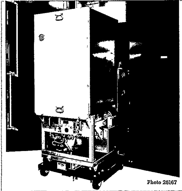
Fig. 5. The breaker is moved out until the guide bar on its bottom touches the front stop on the dolly. Before moving dolly make sure that breaker locking lever is in extreme right position.
